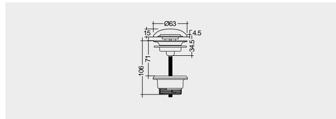
Ceramic Click-Clack Pop-Up Waste DUO000514A Ceramic Free-Flow Waste DUO002514A
